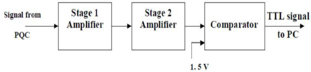
Fig.(3): Block diagram of APD receiver
