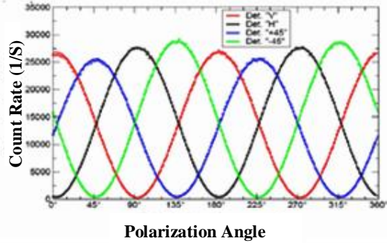
Fig. (2): Variation of detectors count rates with variation of the HWP angle [9]
