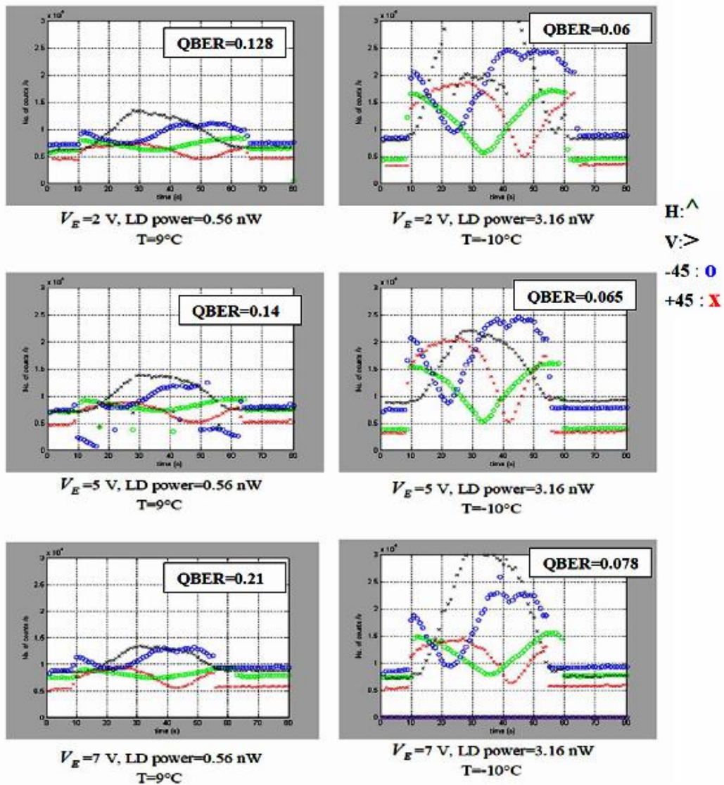
Fig. (5): APDs count at various conditions
