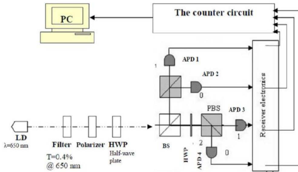
Fig. (4): Optical setup to calculate QBER
