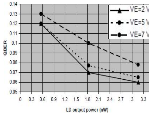
Fig. (7): A comparison of calculated QBER at T=-10^\circ\text{C}
